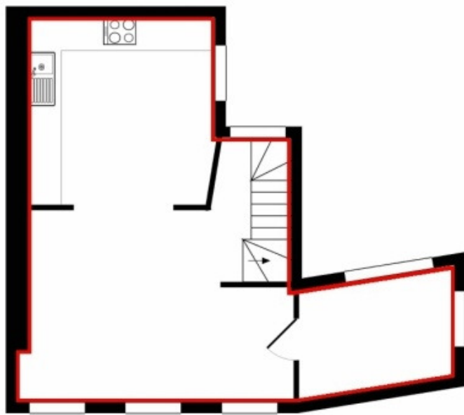
1ST FLOOR
